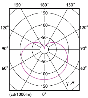
LEDbulb A19 12,2W E26 1100lm 927 FR
